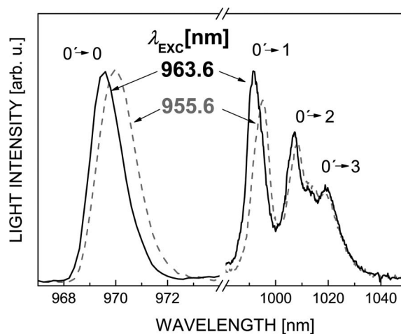
FIG. 5. 5 K photoluminescence spectrum of \text{NaLu}/\text{Yb}_x\text{W} ( x_{\text{melt}}=0.005 ).
