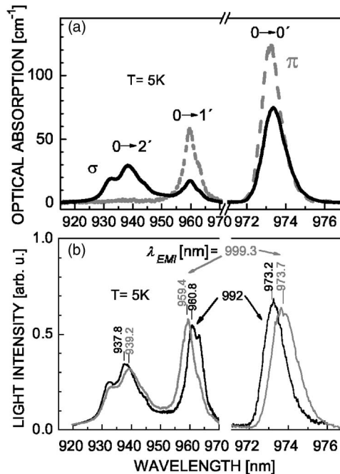
FIG. 4. 5 K polarized optical absorption spectra of \text{NaLu}/\text{Yb}_x\text{W} ( x_{\text{melt}}=0.1 ) (a) and 5 K excitation spectra of \text{NaLu}/\text{Yb}_x\text{W} ( x_{\text{melt}}=0.005 ) (b).
