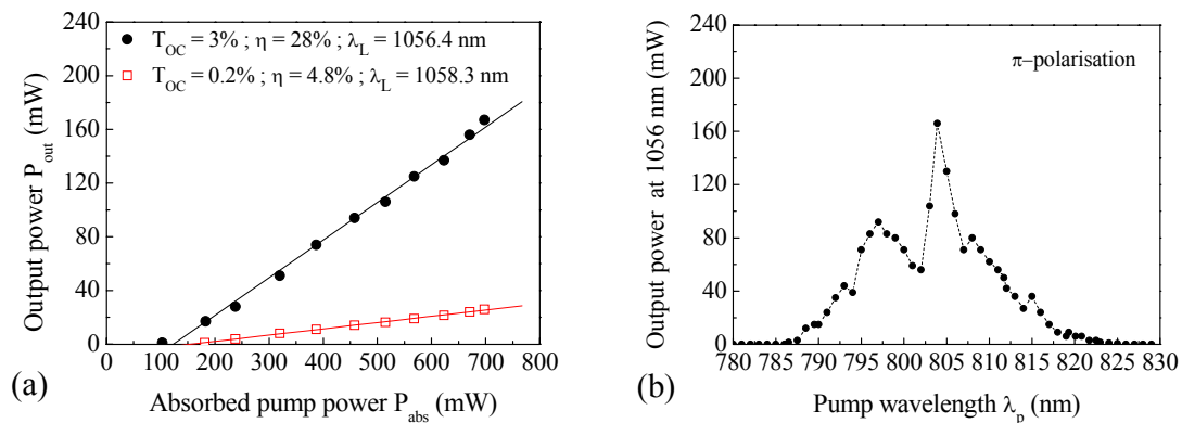
Fig1. (a) Output power ( P_{out} ) versus absorbed pump power ( P_{abs} ) (symbols) of the Nd 3+ :NaLaW laser obtained for E//c. The linear fits give the slope efficiencies \eta for both used T_{OC} . (b) \pi -polarised output power versus pump wavelength for an incident pump power ( P_{inc} ) of 740 mW and T_{OC} = 3\% at 1056 nm (filled circles), is shown.
