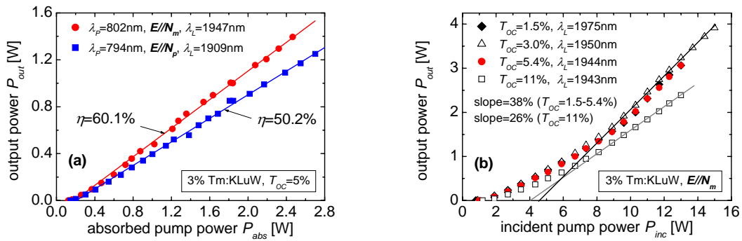
Fig. 1. Input-output characteristics of the Ti:sapphire laser pumped Tm:KLuW laser for two polarizations in terms of absorbed pump power (a) and input-output characteristics of the diode laser pumped Tm:KLuW laser for E//N_m in terms of incident pump power (b).
